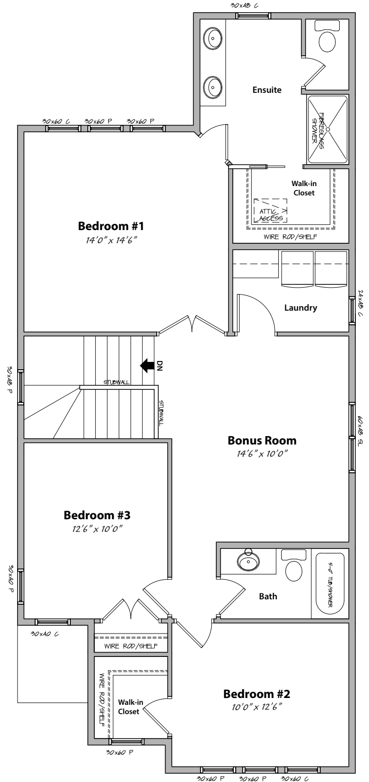
Second Level 1070 sq.ft.
