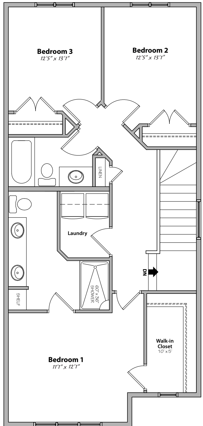
Second Floor 782 sq.ft.
