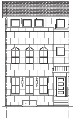
Front Elevation 1,766 sq. ft.
