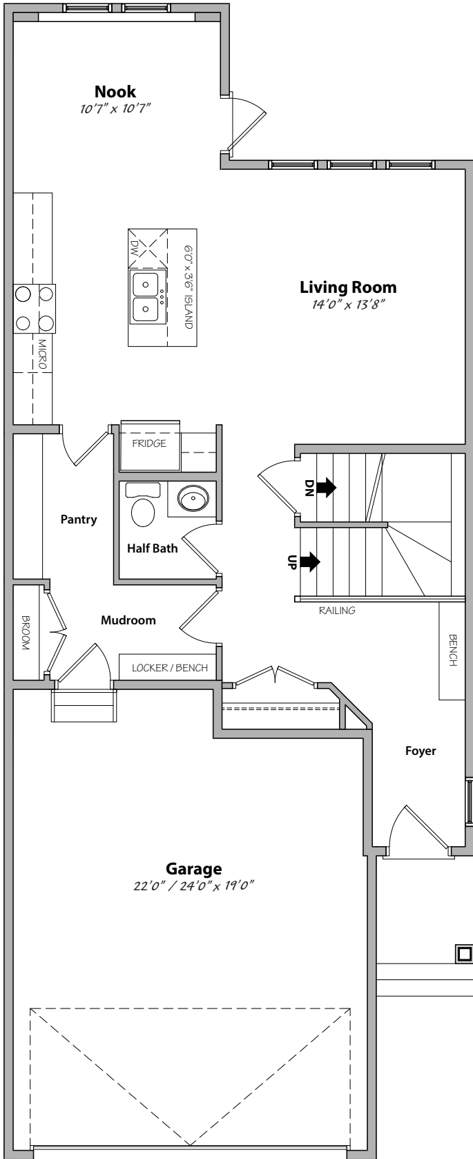
Main Floor 808 sq.ft.
