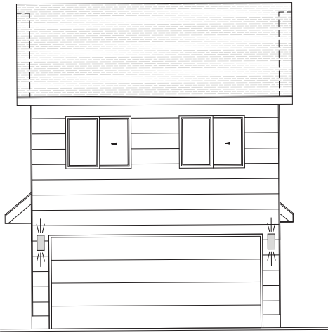
Front Elevation
