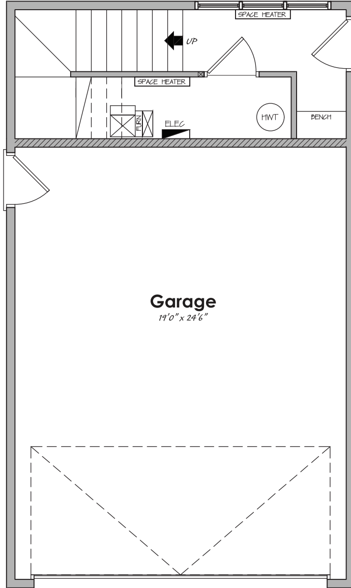
Garage Level Plan 607 sq. ft.
