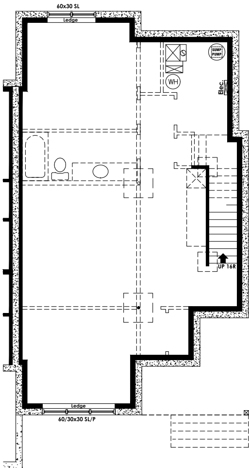
Basement Plan
